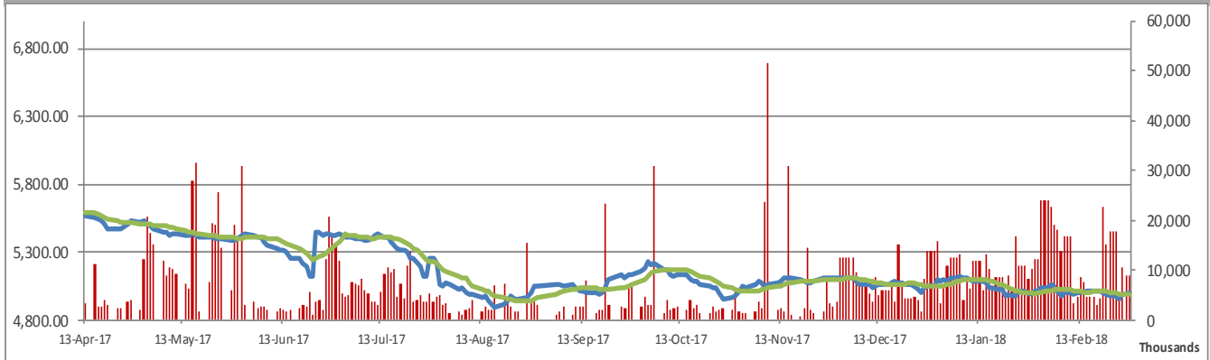
MSM 30 one year close (In Blue) & turnover (In Red) Vs MA10 (In Green)
